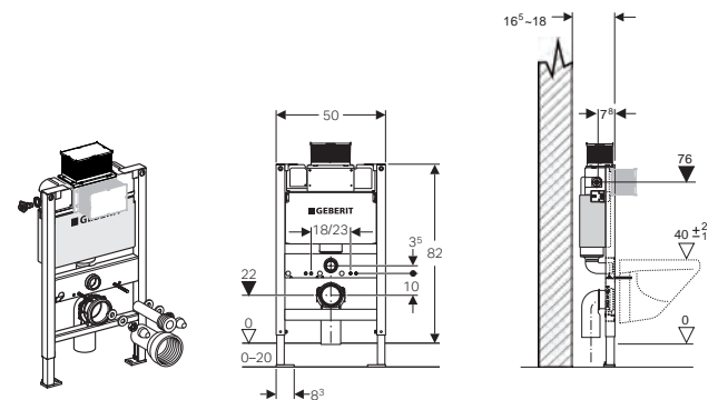
Duofix element with Kappa concealed cistern, thickness 150mm, height 820mm
